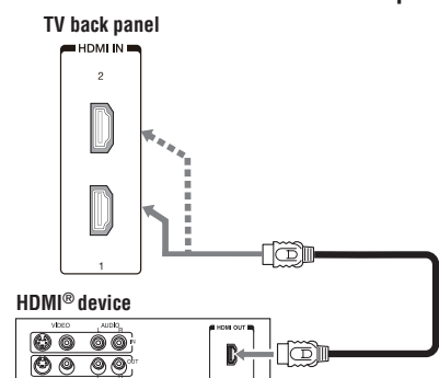
(Sample Illustration) Connecting an HDMI® device
